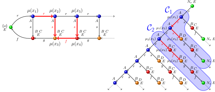
Fig. 2. Correspondence between entailment and quantailment. Left: match \mu for q = \{r(x_1, x_2), s(x_2, x_3), f(x_4, x_3), s(x_5, x_4)\} into the “proper model”. Right: anchored components \mathcal{C}_1 and \mathcal{C}_2 and functions \mu_1 and \mu_2 establishing \downarrow(\mathcal{I}) \approx q .
