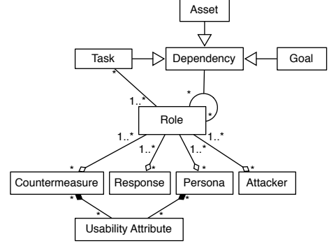
Figure 4: Responsibility Meta-Model
