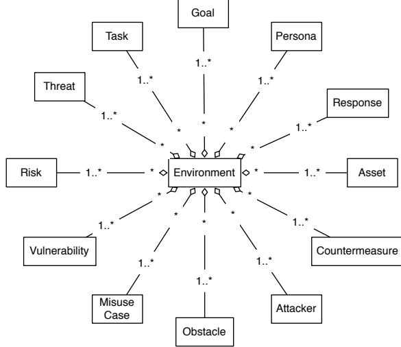
Figure 5: Environment Meta-Model
