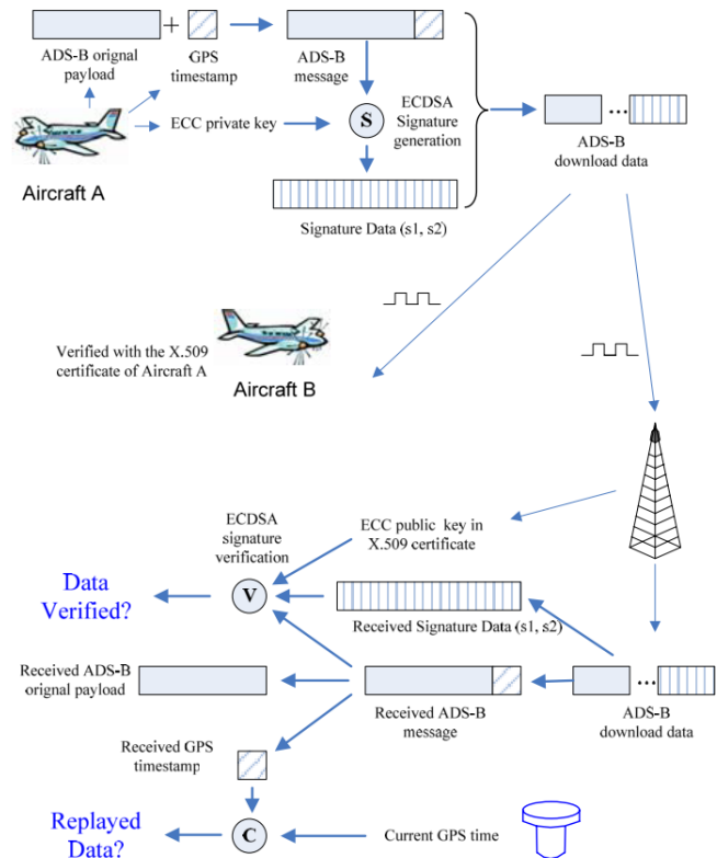
Figure 8. Example of a typical encryption scheme adapted for ADS-B from [71]. It employs elliptic curve cryptography to generate signatures which can be verified with the responding certificate by other aircraft and ground stations. An additional GPS timestamp prevents replay attacks.
