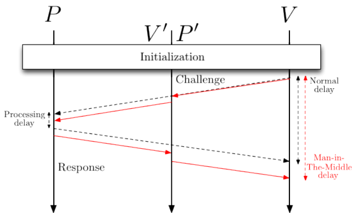
Figure 14. Principle of distance bounding protocols. The verifier V sends a challenge to the prover P who then, after processing, sends his response (black dashed arrows). A man in the middle ( V'/P' ) can only increase the distance by adding further processing delays, but not decrease it (red arrows).
