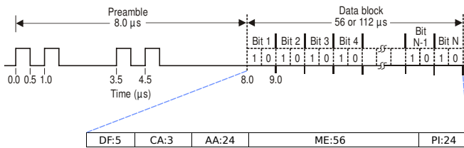
Figure 3. 1090 ES Data Link [9]
