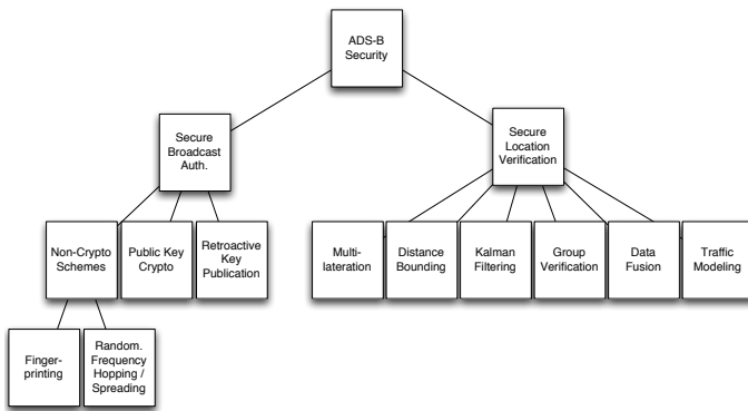
Figure 4. Taxonomy of ADS-B Security
