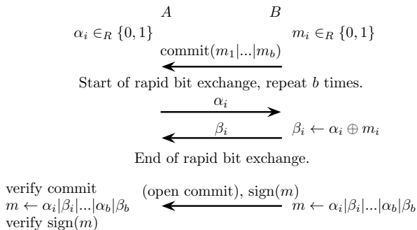
Figure 15. Original untrusting distance bounding protocol by Chaum and Brands [96]. A is the verifier, B the prover. After the protocol exchange A can verify that B is within a given distance.
