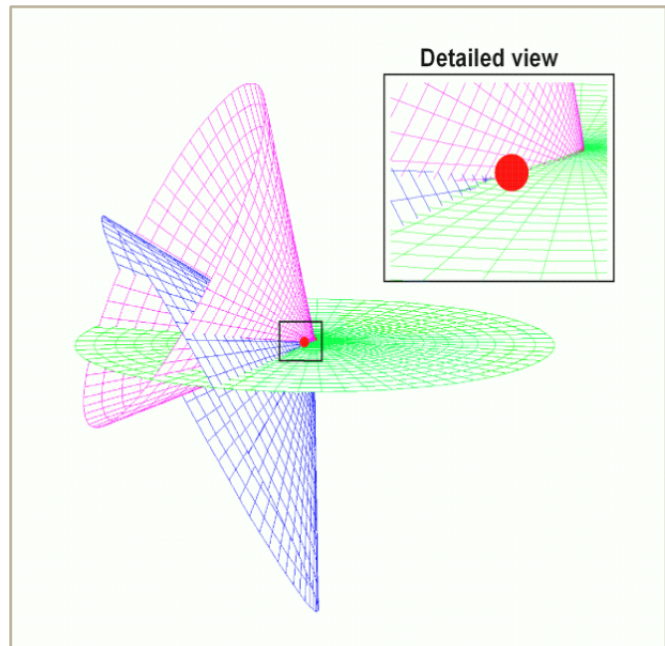
Figure 11. Intersection of three hyperboloids from [87]. With four receivers in a 3D setting, one can specify the origin of the message as the red point where the computed hyperboloids intersect.
