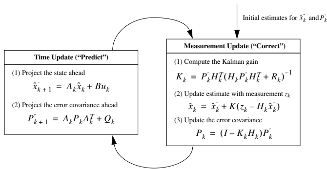
Figure 17. Basic concept of Kalman filtering from [105]. The time update step projects the measured variables and the error covariances. The measurement update step computes the Kalman gain and updates the estimates and error covariances with the actual measurements.
