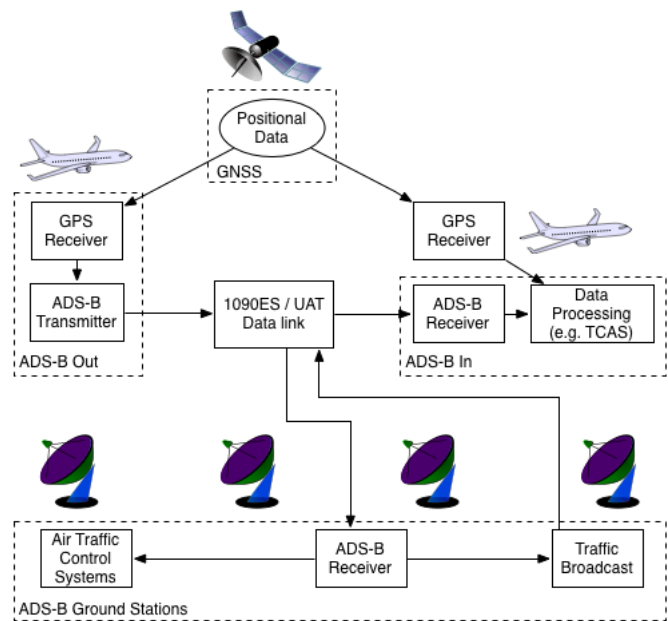
Figure 2. Overview of the ADS-B system architecture. Aircraft receive positional data that is transmitted via the ADS-B Out subsystem over the 1090ES or the UAT data link. It is then received and processed by ground stations and by other aircraft via the ADS-B In subsystem.
