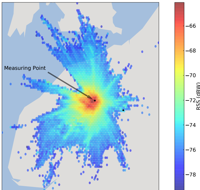
Figure 21. Example of an RSS heat map used for traffic modeling from [9]. The colors indicate the received signal strength at a single measuring point which correlates strongly with the distance. Though it is relatively easy for an attacker to manipulate the RSS, it becomes increasingly difficult the more measuring points have to be deceived.
