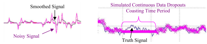
Figure 18. Example of Kalman filtering from [107]. Noisy signals are being smoothed (left), dropped data being coasted over below a given cutoff point (right).
