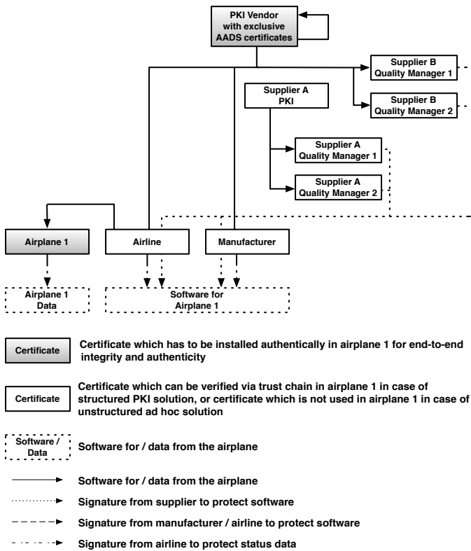
Figure 7. Outline of a potential public key infrastructure after [70]. A PKI vendor supplies airlines, manufacturers and external suppliers with the required certificates.
