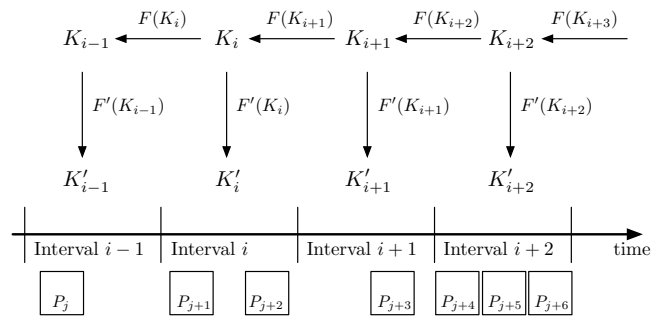
Figure 9. The figure illustrates TESLA’s utilization of one-way chains after [78]. The first one-way function F generates the chain, following that the second one-way function F' derives the MAC keys. Time is divided into separate intervals i , all having the same length. The packets P_j are each sent during one specific interval. For every such packet, the sender computes a MAC with the key that is in accordance with that interval. E.g. P_{j+2} ’s MAC is calculated based on its data and key K'_i . Disclosing the keys of previous intervals can be done either by attaching the key to sent packets or in separate messages.
