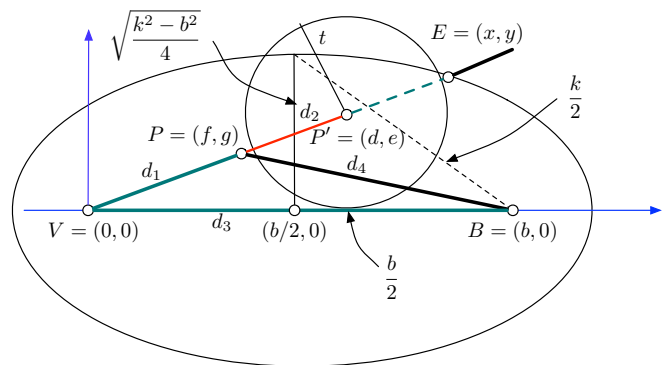
Figure 16. Network topology for a minimum distance guarantee after [99]. V is the verifier, P the prover, P' its claimed location. B is a common neighbour of both V and P who gives an estimate E of P 's position. Considering the ellipse and a certain error distance, B can detect the distance enlargement of P .
