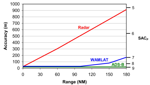
Figure 13. Comparison of location estimation accuracies when utilizing primary radar, wide area multilateration and ADS-B [14]. SAC_p denotes the Surveillance Accuracy Category for Position as defined in [14].
