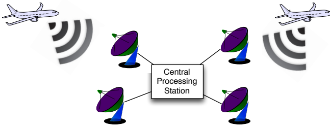
Figure 12. Basic multilateration architecture. Four (or more) receiver stations measure the time at which they receive the same message from an aircraft. They send this data to the central processing station which can calculate the aircraft's position from the time difference of arrival between the receiver stations.
