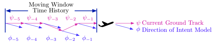
Figure 19. Practical application of intent verification in ADS-B from [107]. The example analyzes the horizontal aircraft motion with a global correlation function as a moving window over local correlation functions.
