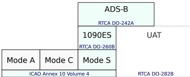
Figure 1. ADS-B hierarchy [9]. The 1090 MHz Extended Squitter is based on the traditional Mode S system and provides the data link for ADS-B in commercial aviation. UAT is a new development but currently only mandated for general aviation.
