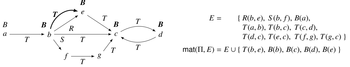
Figure 1: The dataset and the materialisation from Example 1. Constants correspond to vertices; explicit facts are shown in normal font, and facts introduced by materialisation are shown in bold font; unary facts are shown by labelling constants with predicates; and binary facts are shown as arcs labelled with predicates.
