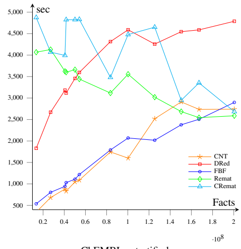
ChEMBL R stratified (four cases: FBF and CNT similar, and they outperform DRed)
