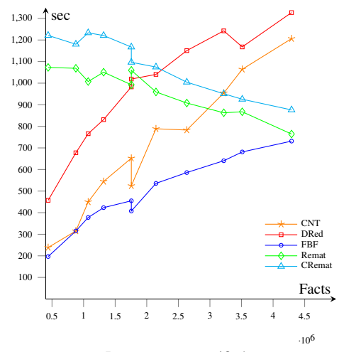
Reactome R unstratified (five cases: FBF outperforms CNT, which outperforms DRed)
