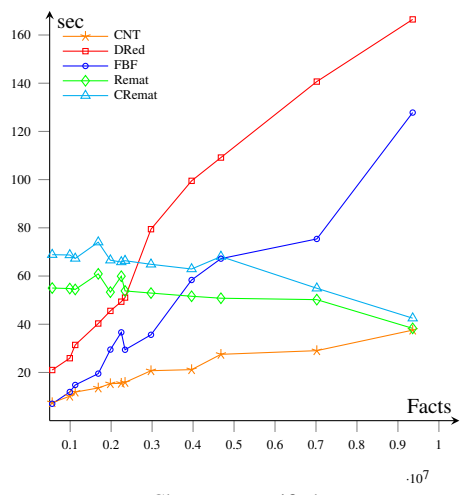
Claros L unstratified (six cases: CNT outperforms FBF, which outperforms DRed)
